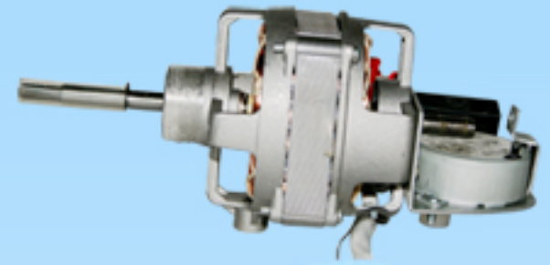
KM-16 Fan Motor with synchronous Motor
